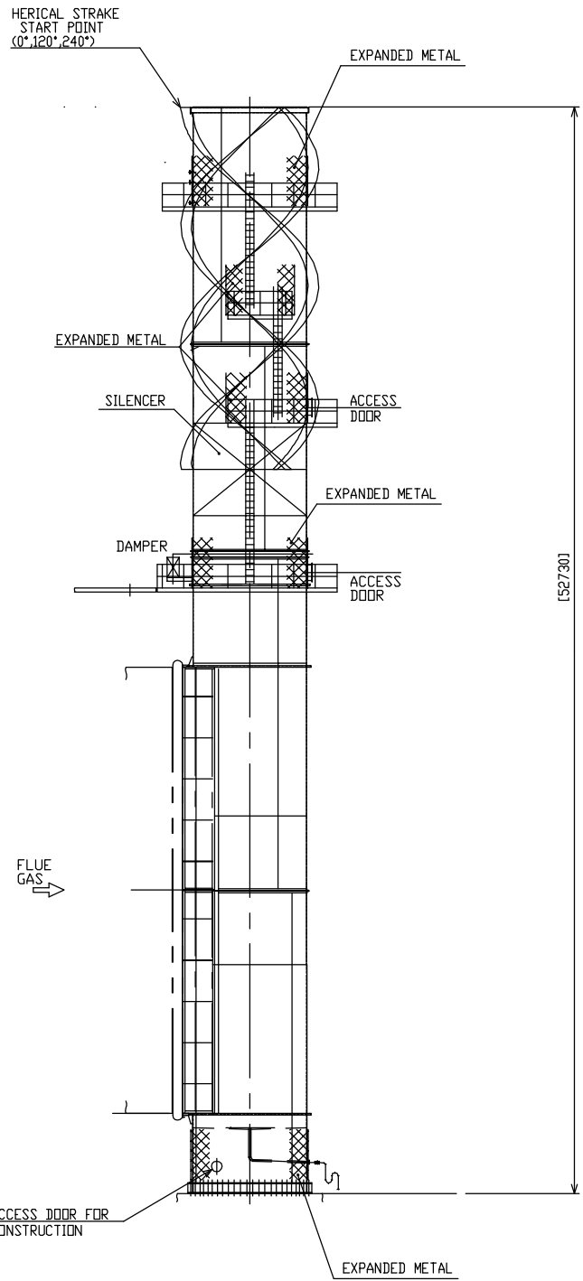
STACK ASSEMBLY
